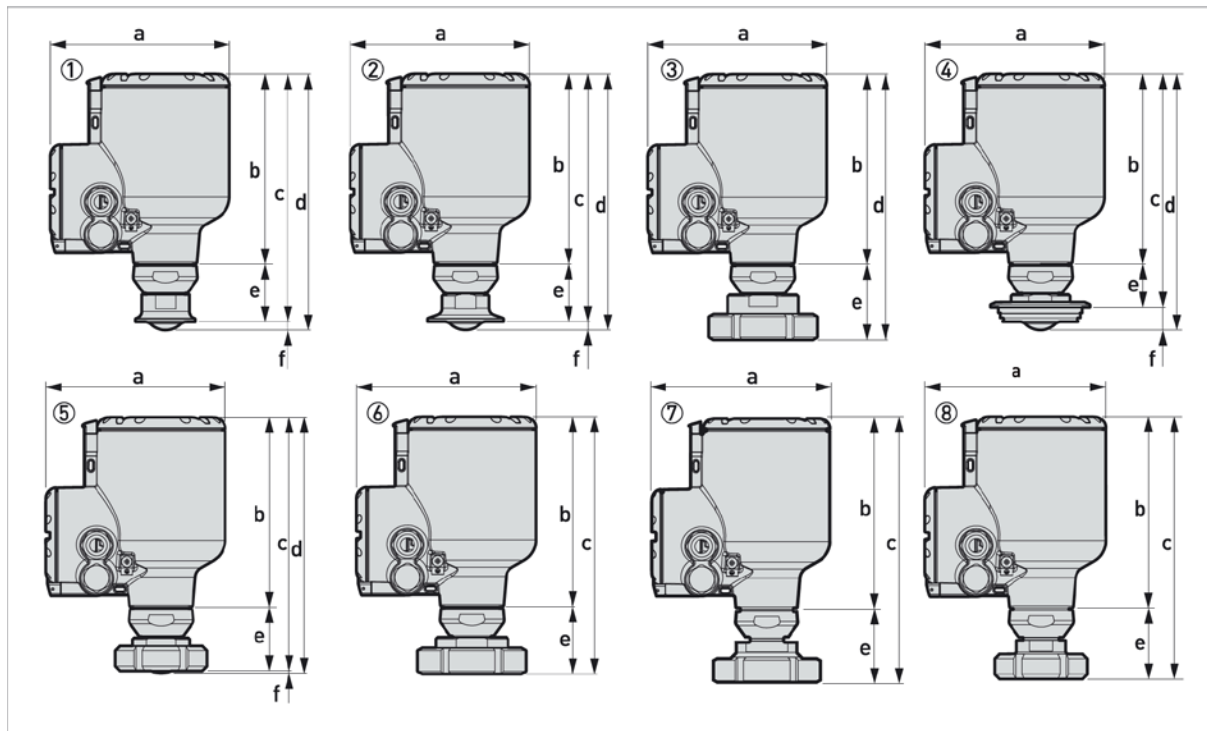
Figure 2-7: DN25 / 1" Lens antenna versions
