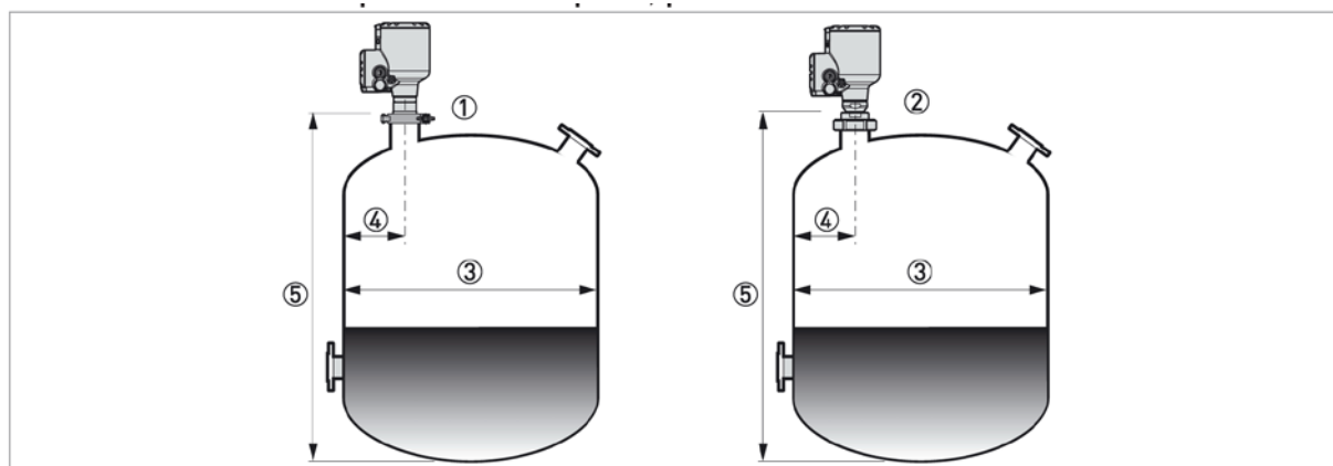
Figure 3-2: Recommended nozzle position for solids
