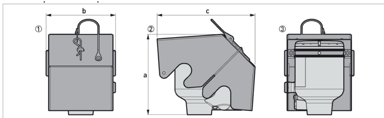
Figure 2-9: Weather protection option
