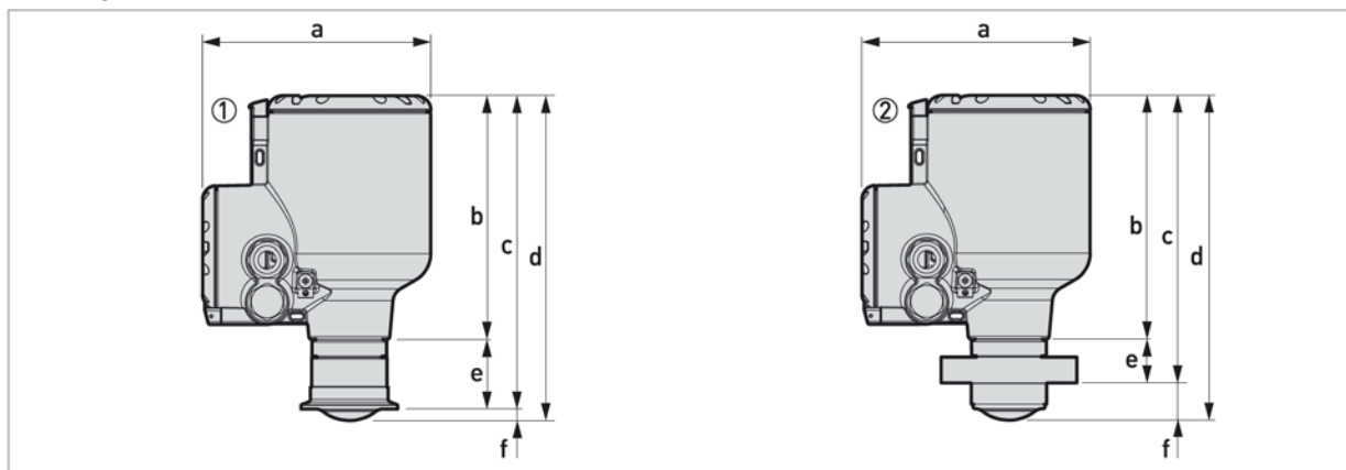
Figure 2-8: DN40 / 1½" Lens antenna versions
