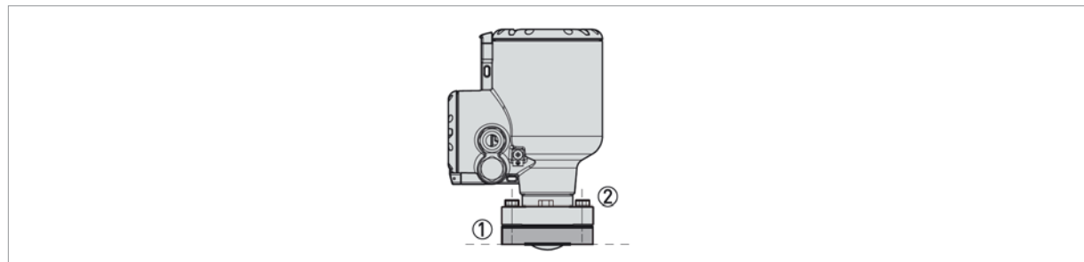
Figure 3-6: BioControl® connection: installation procedure BioControl® connection on the tank Flange bolts
