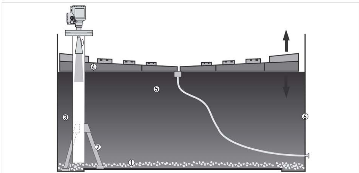
Figure 3-11: Floating roofs
