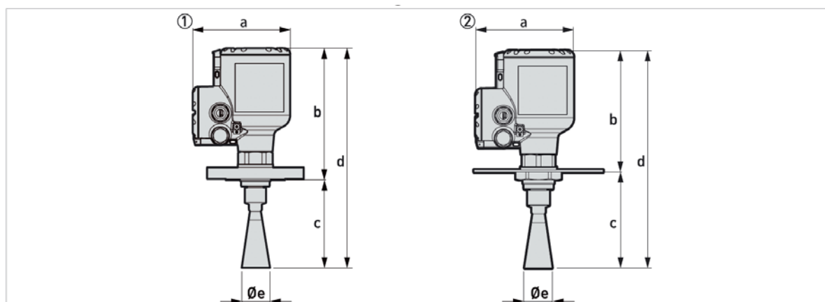
Figure 2-10: Metallic Horn antennas with flange connections
