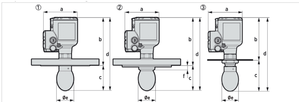
Figure 2-12: Drop antennas with flange connections
