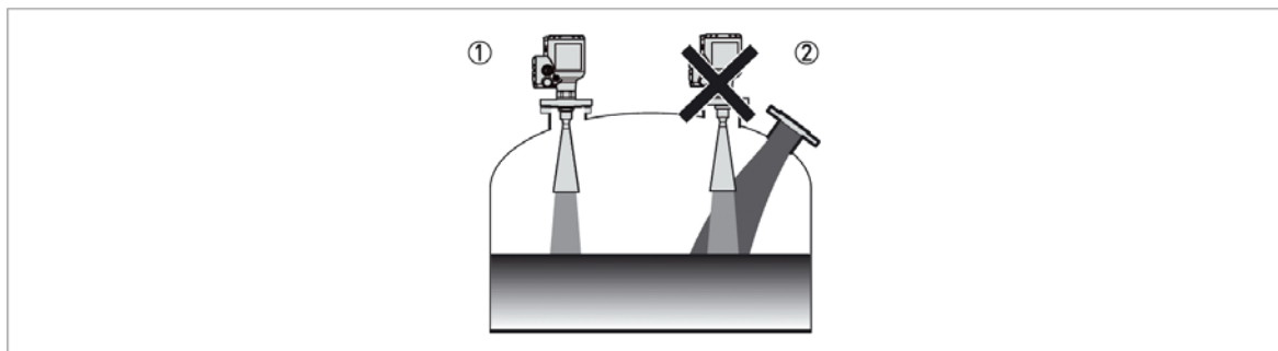
Figure 3-5: Product inlets
