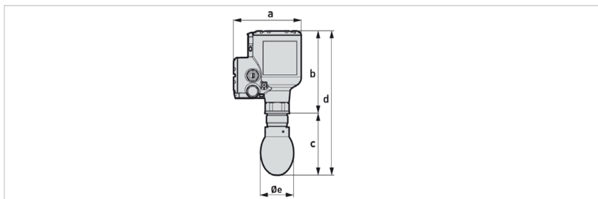
Figure 2-11: Drop antennas with threaded connections
