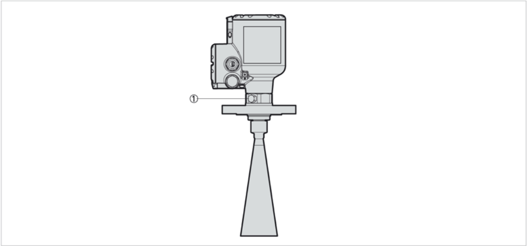
Figure 2-13: Purging options
