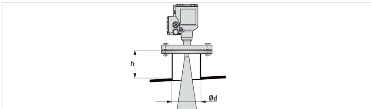
Figure 3-6: Flange connections
