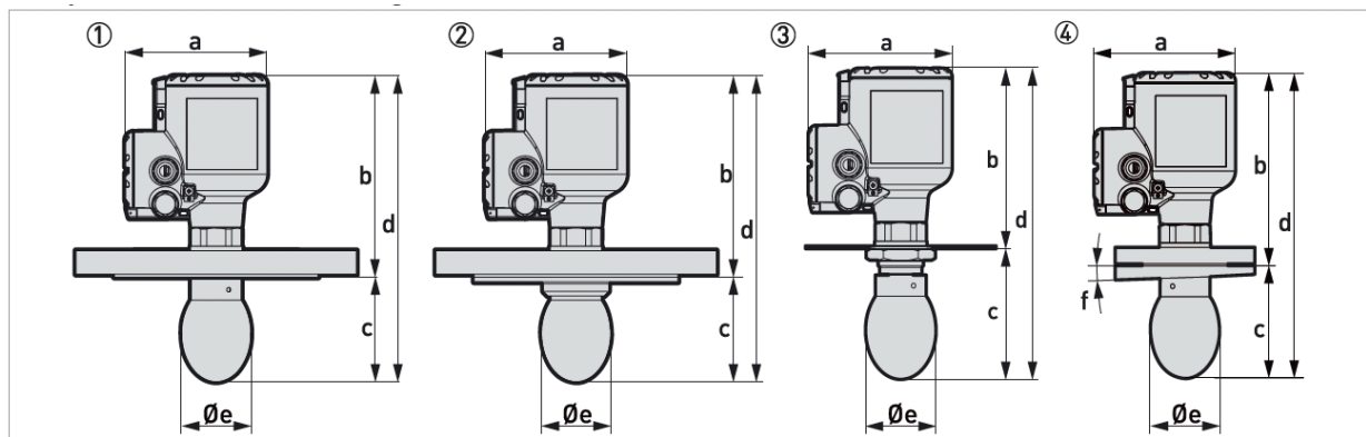
Figure 2-12: Drop antennas with flanged connections
