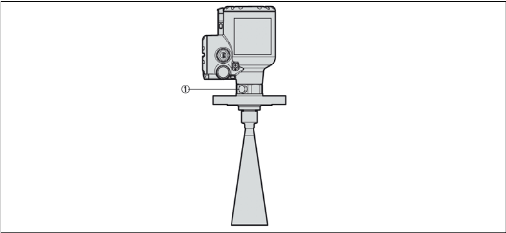
Figure 2-13: Purging option ① G 1/4 threaded connection for purging system (the plug is supplied by the manufacturer)
