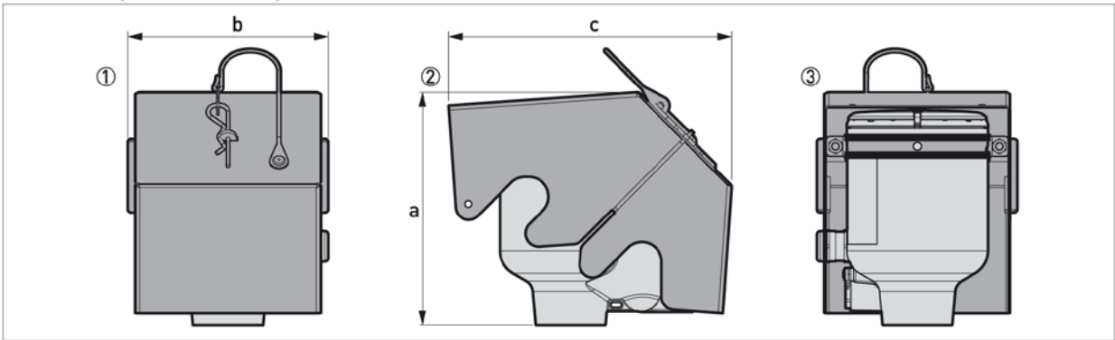
Figure 2-14: Weather protection option ① Front view (with weather protection closed) ② Left side (with weather protection closed) ③ Rear view (with weather protection closed)
