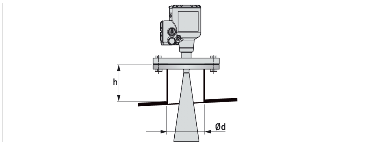
Figure 3-6: Flange connections
