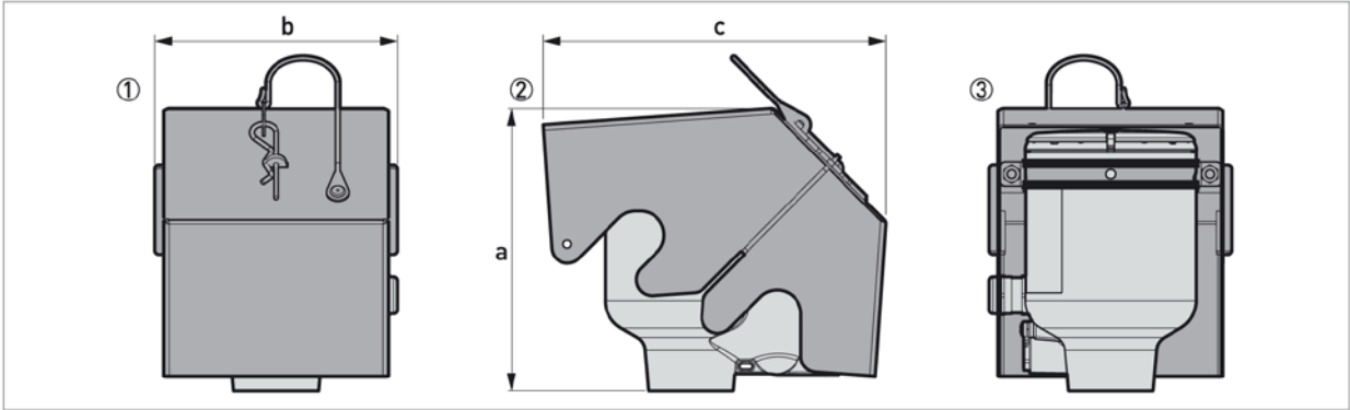
Figure 2-13: Weather protection option
