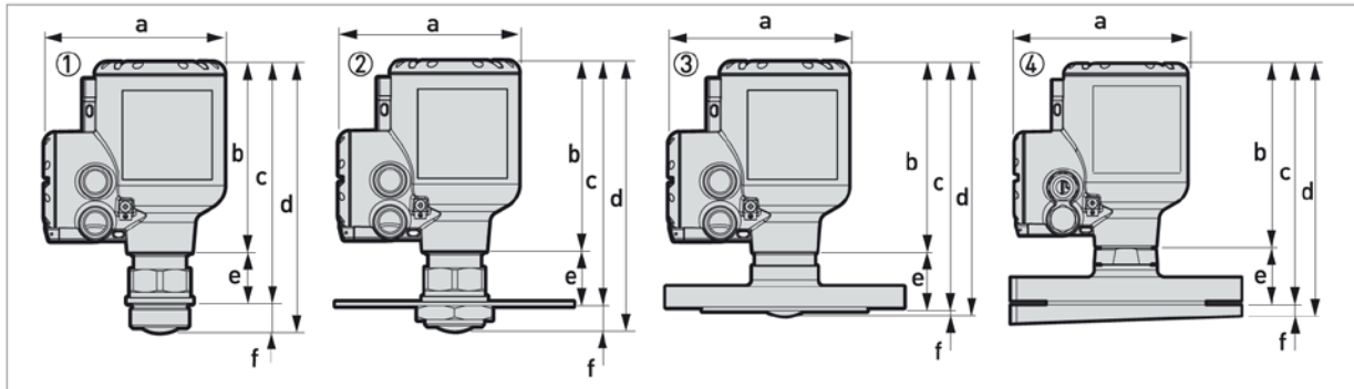
Figure 2-11: DN40 / 1½" Lens antenna versions
