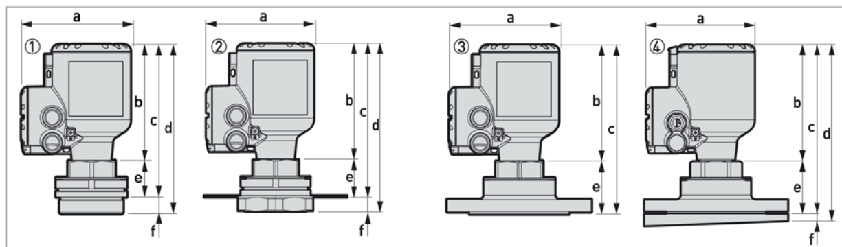
Figure 2-12: DN70 / 2¾" Lens antenna versions
