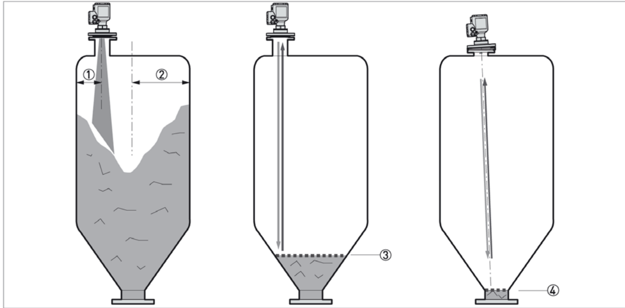
Figure 3-2: Recommended nozzle position for solids
