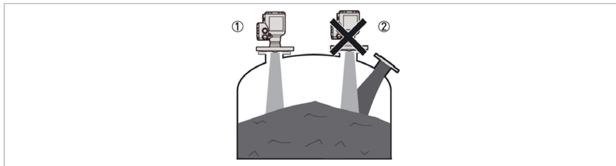
Figure 3-5: Product inlets
