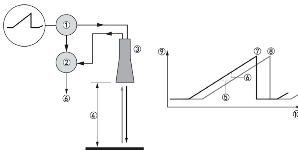
Figure 1-1: Measuring principle of FMCW radar
