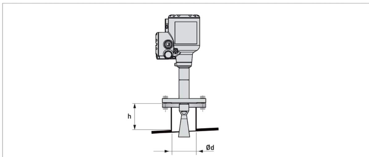
Figure 3-6: Flange connections
