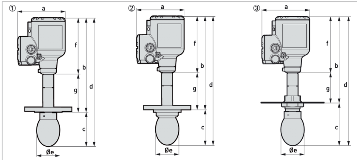
Figure 2-12: Drop antennas with flanged connections
