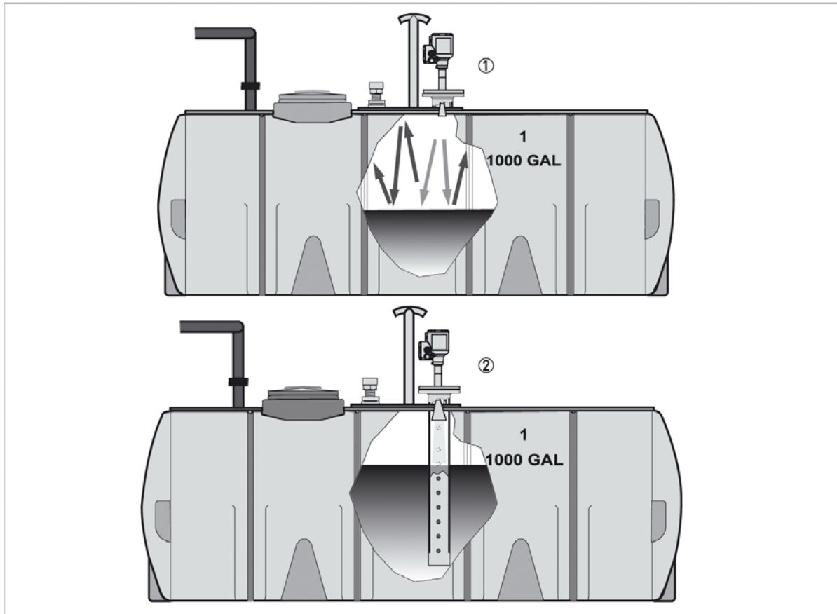
Figure 3-12: Horizontal cylindrical tanks
