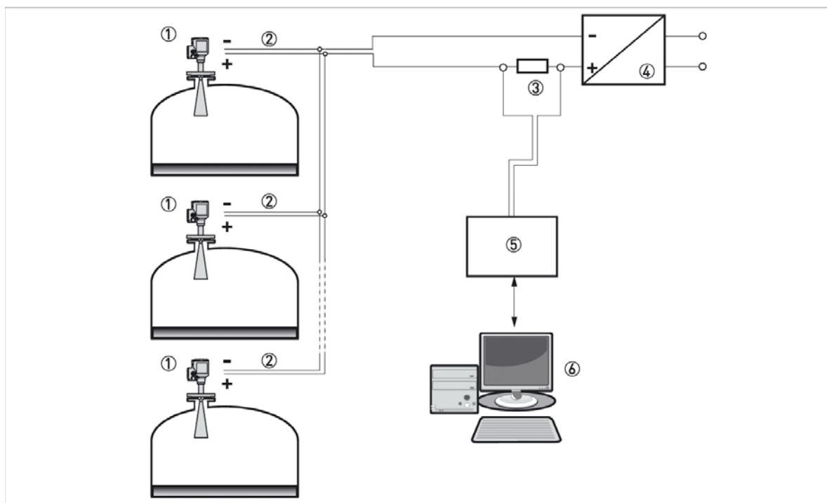
Figure 4-4: Multi-drop network (non-Ex)
