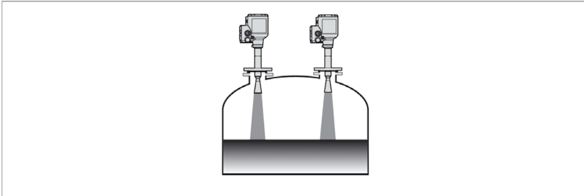
Figure 3-3: There is no maximum limit to the number of devices that can be operated in the same silo
