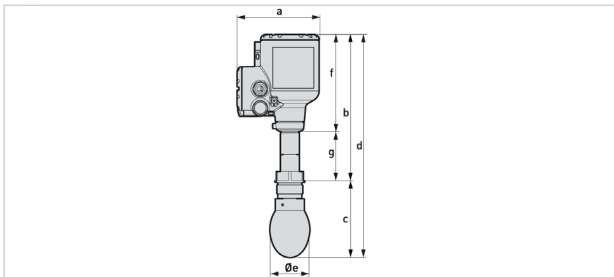
Figure 2-11: Drop antennas with threaded connections
