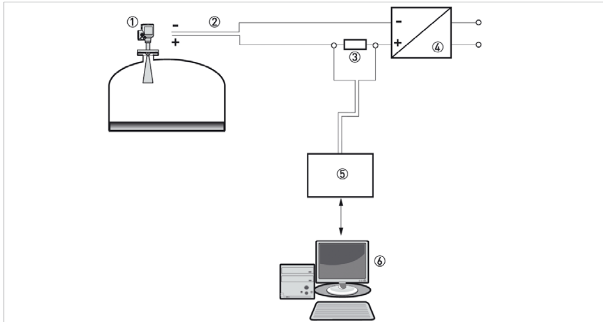
Figure 4-3: Point-to-point connection (non-Ex)
