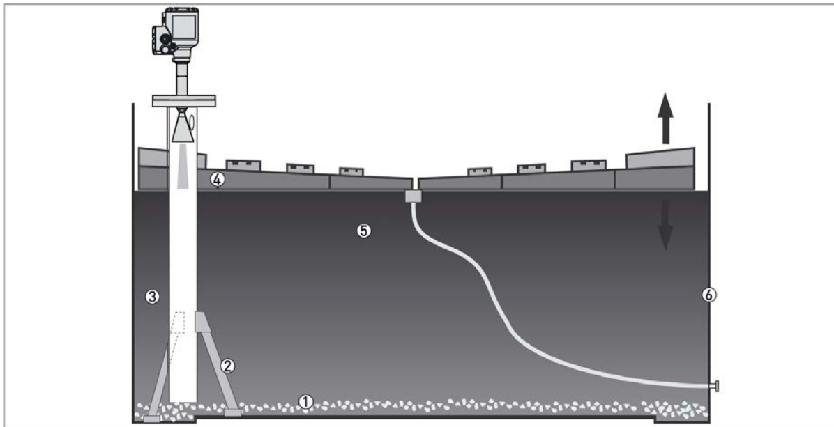
Figure 3-11: Floating roofs
