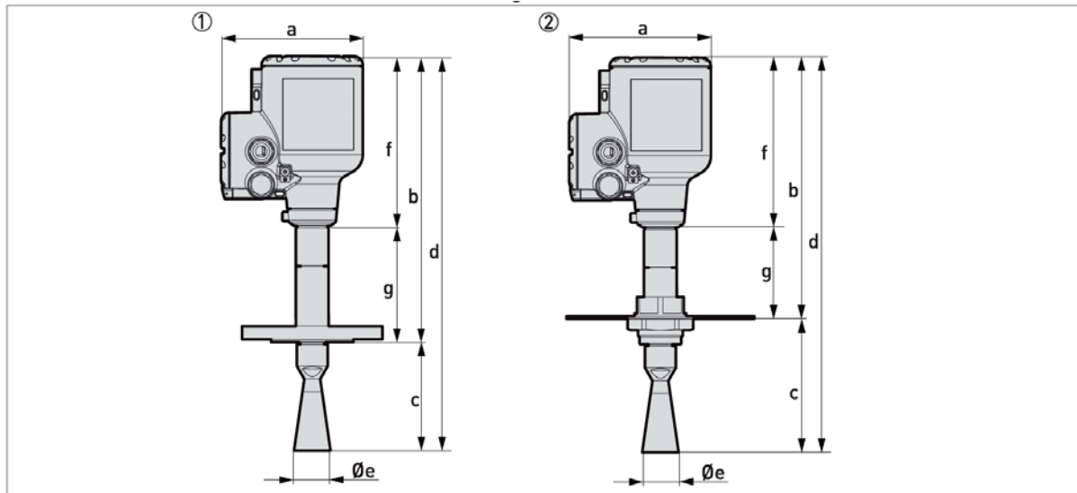
Figure 2-10: Metallic Horn antennas with flange connections
