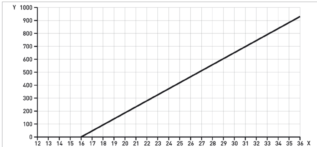
Figure 2-10: Minimum power supply voltage for an output of 21.5 mA at the terminal (Hazardous Location approval (Ex d / XP/NI))
