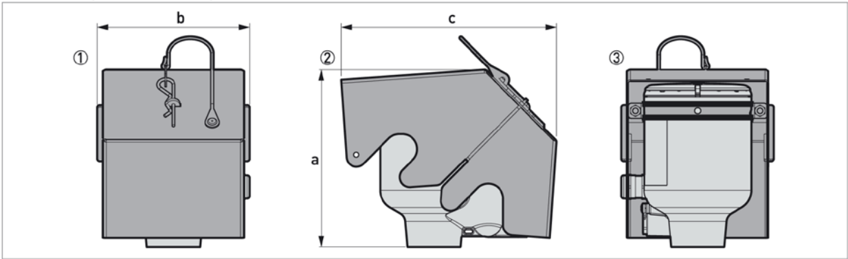
Figure 2-19: Weather protection option
