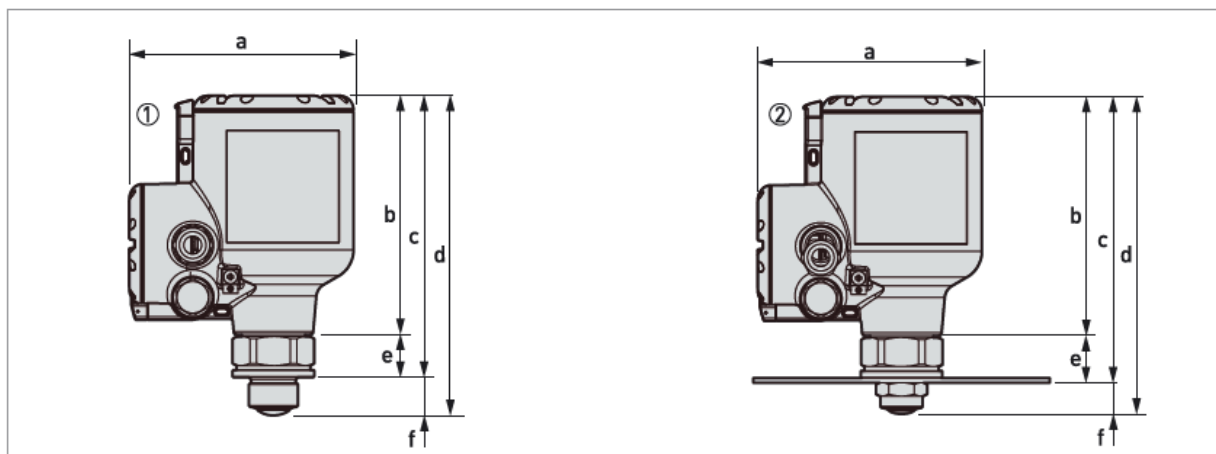
Figure 2-16: DN25 / 1" Lens antenna versions
