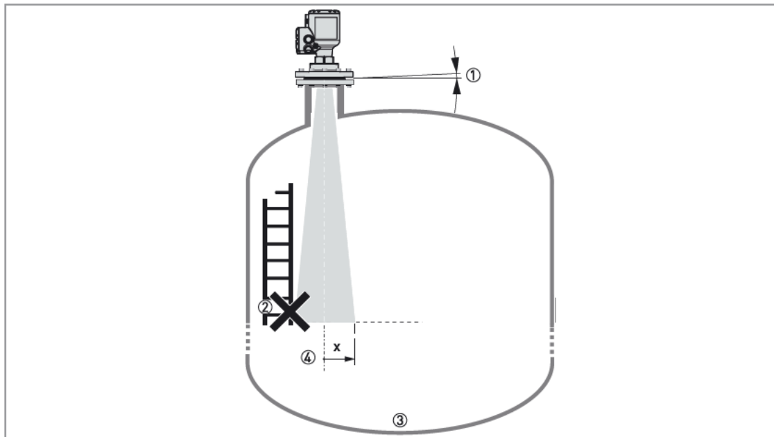
Figure 3-4: Equipment and obstacles: how to prevent measurement of interference signals
