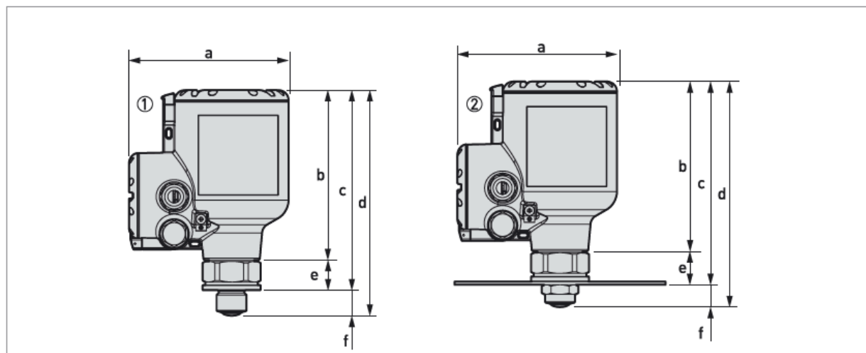
Figure 2-15: DN20 / 3/4" Lens antenna versions
