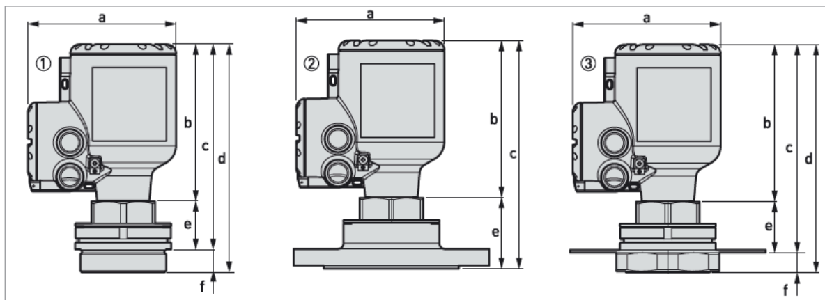
Figure 2-18: DN70 / 2¾" Lens antenna versions
