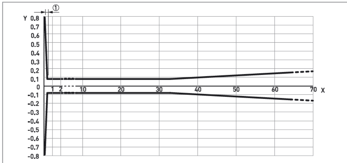
Figure 2-2: Figure 2-2: DN20 (¾") Lens antenna: measuring accuracy (graph of measuring accuracy in inches against measuring distance in ft)
