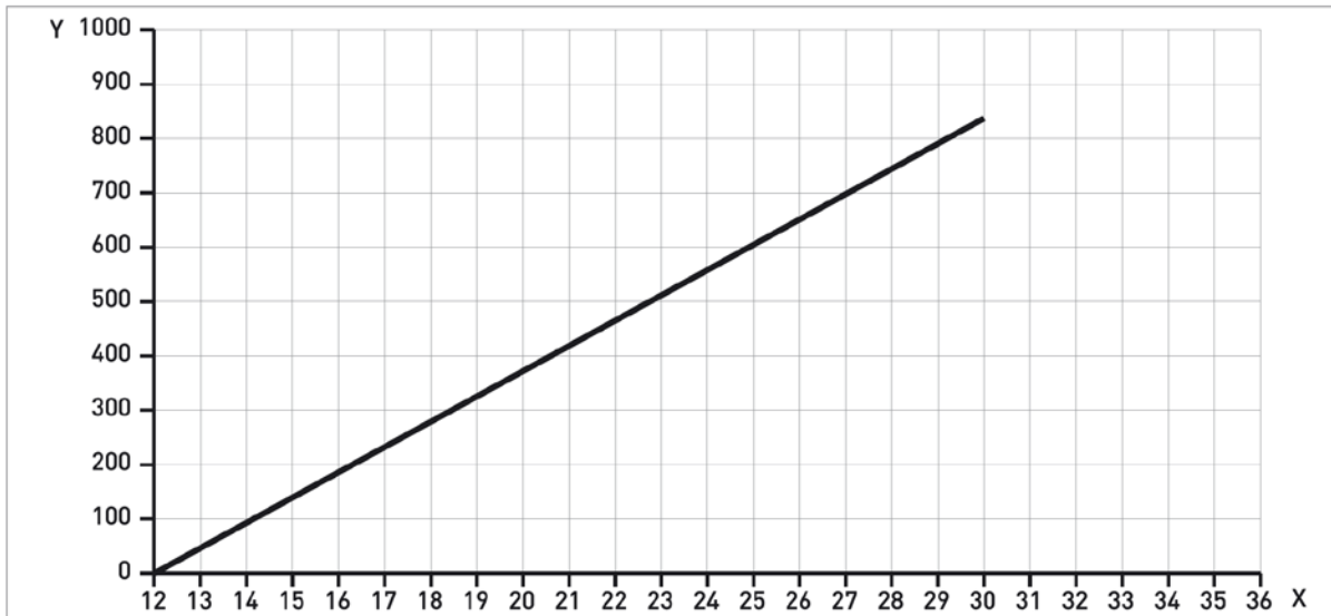
Figure 2-9: Minimum power supply voltage for an output of 21.5 mA at the terminal (Non-Ex and Hazardous Location approval (Ex i / IS))
