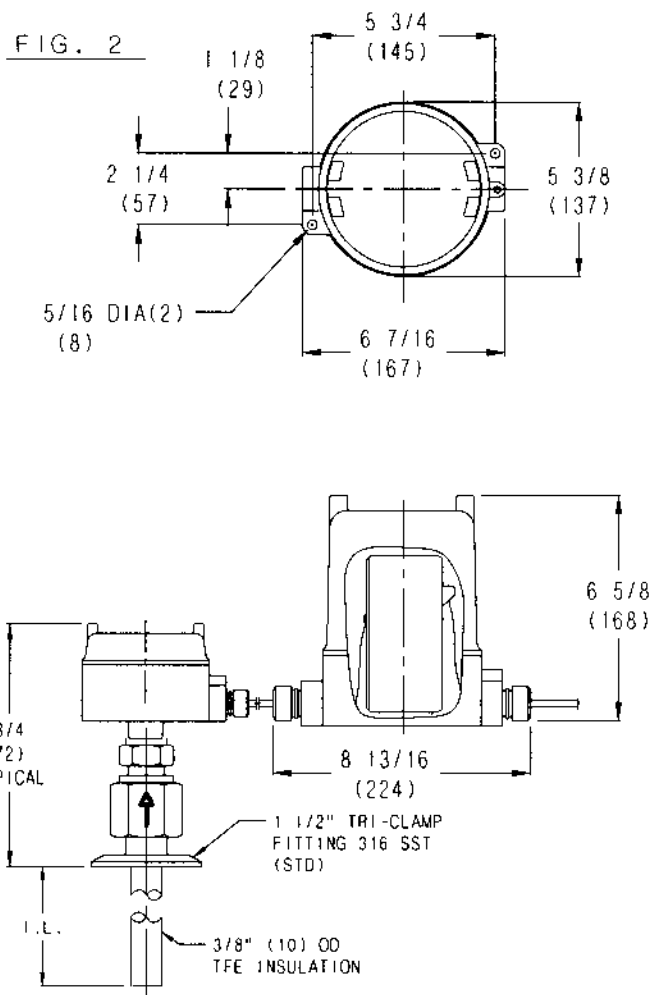
REMOTE MOUNTING OF CHASSIS IN EXPLOSION-PROOF HOUSING
