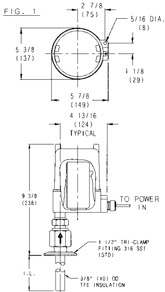
INTEGRAL MOUNTING OF CHASSIS IN EXPLOSION-PROOF HOUSING
