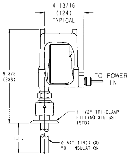
INTEGRAL MOUNTING OF CHASSIS IN EXPLOSION-PROOF HOUSING
